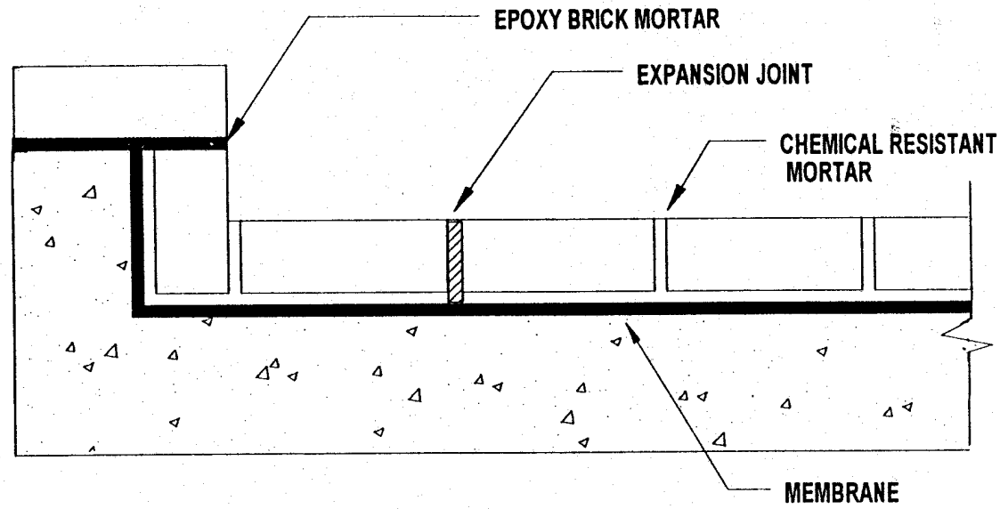
MEMBRANE/BRICK CURBING DETAIL
