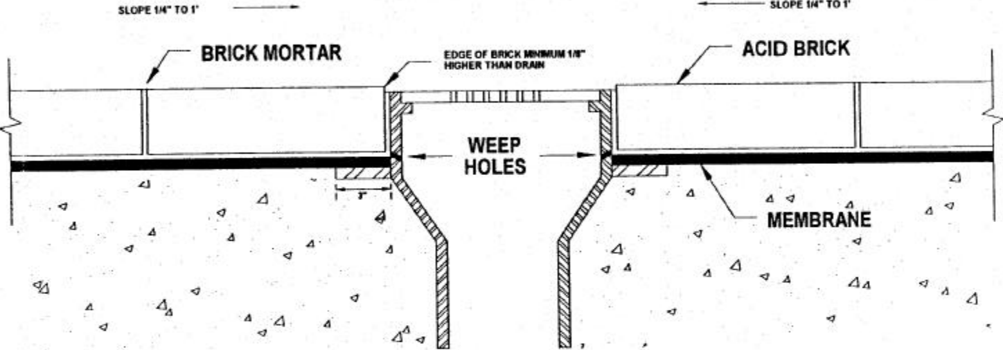
MEMBRANE/BRICK FLOOR DRAIN DETAIL
