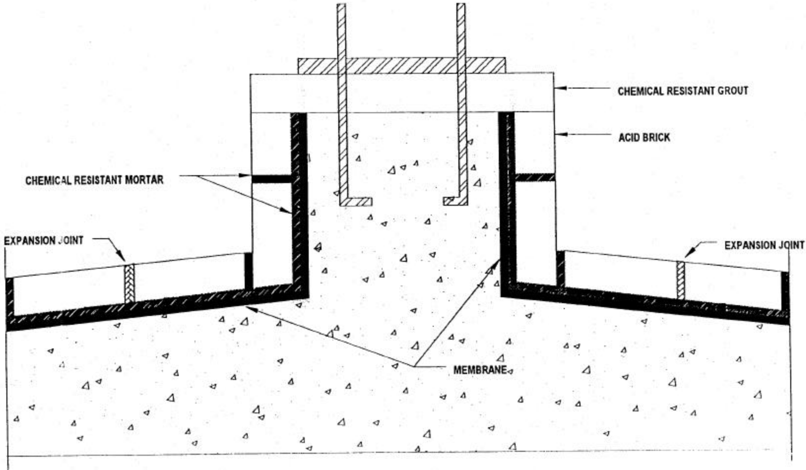
MEMBRANE/BRICK EQUIPMENT BASE WITH GROUT CAP
