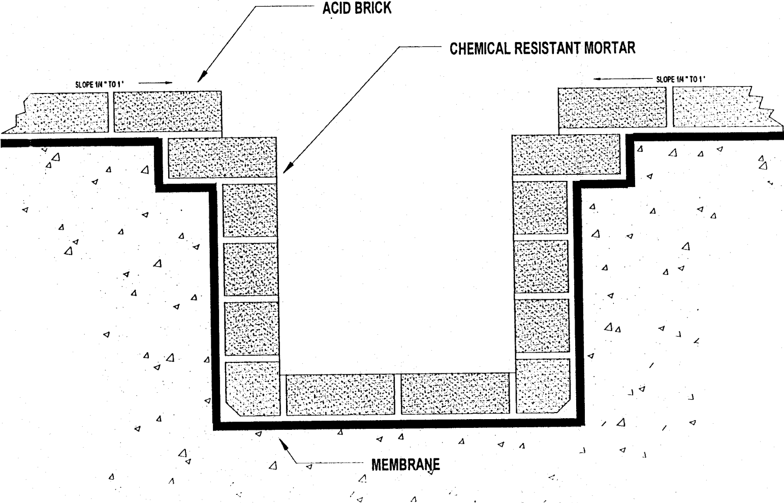
MEMBRANE/BRICK LINED TRENCH/SUMP
