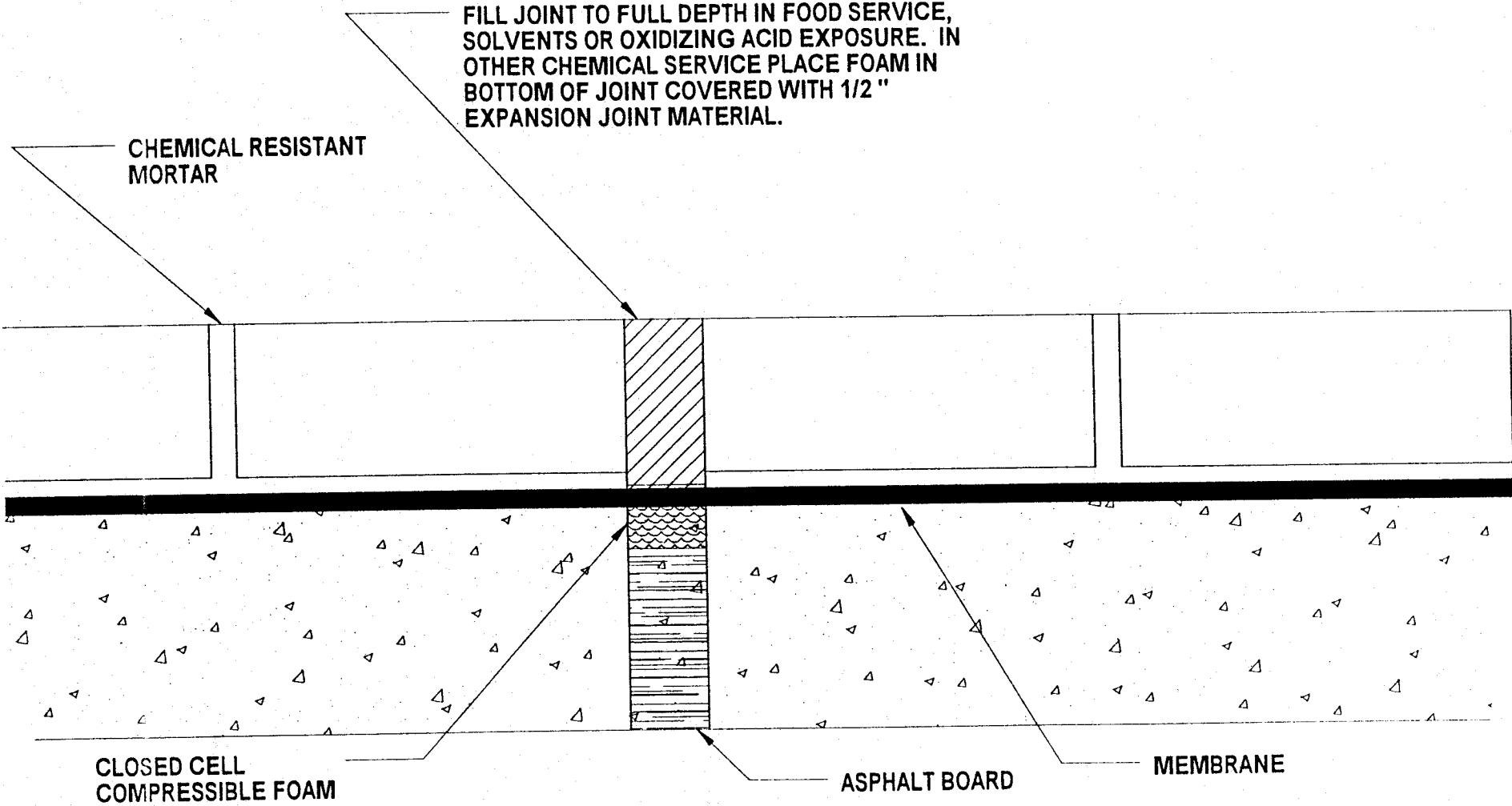
TYPICAL EXPANSION JOINT IN MEMBRANE/BRICK FLOORS
