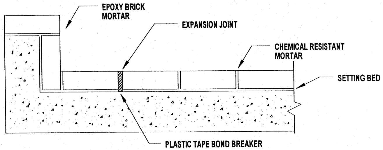
DIRECT BOND CURBING DETAIL
