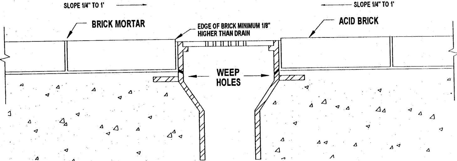
DIRECT BOND FLOOR DRAIN DETAIL
