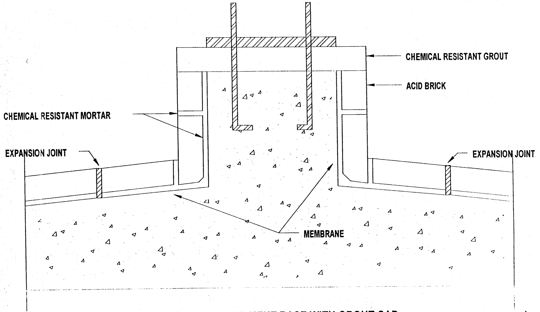
DIRECT BOND EQUIPMENT BASE WITH GROUT CAP
