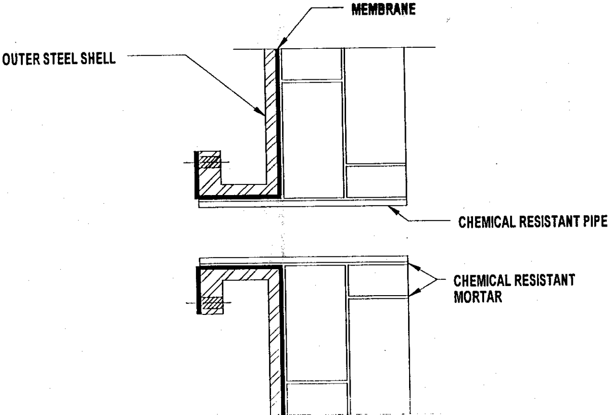
STEEL TANK OUTLET
