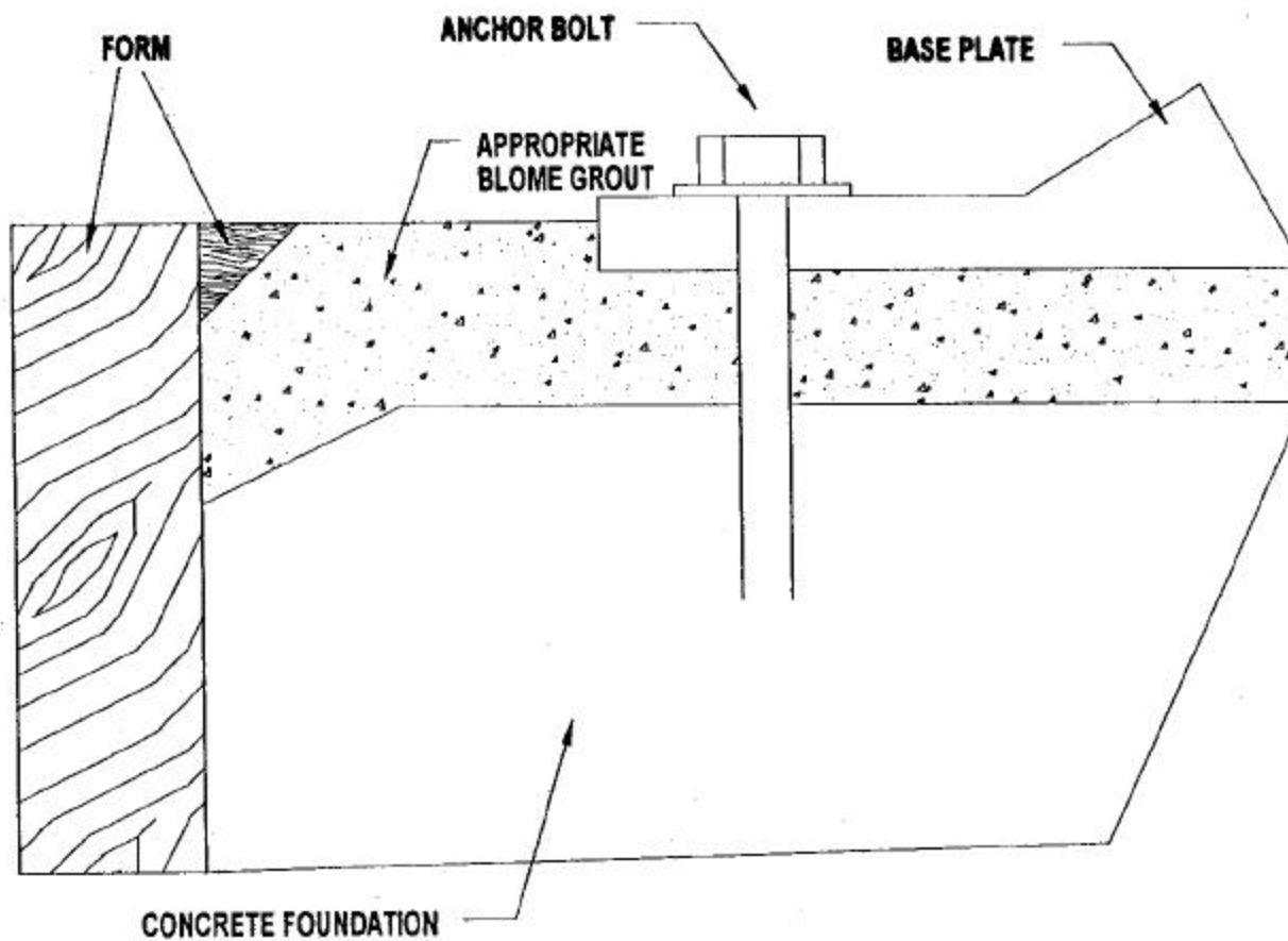
EQUIPMENT BASE PLATE GROUTING DIAGRAM
