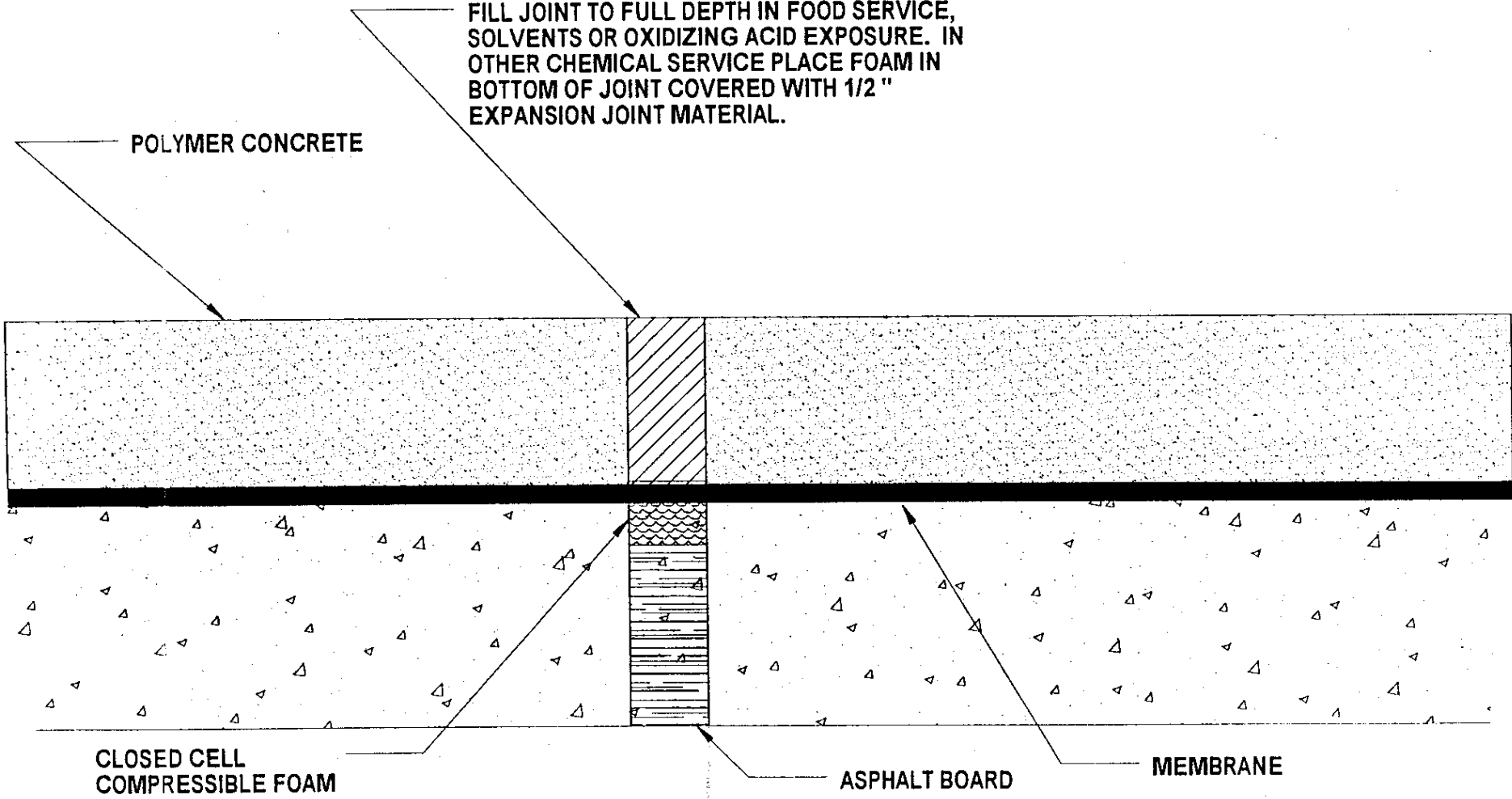
TYPICAL EXPANSION JOINT IN POLYMER CONCRETE FLOORS
