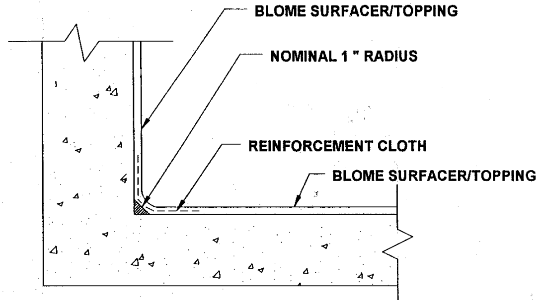
MONOLITHIC TOPPING FLOOR TO WALL DETAIL
