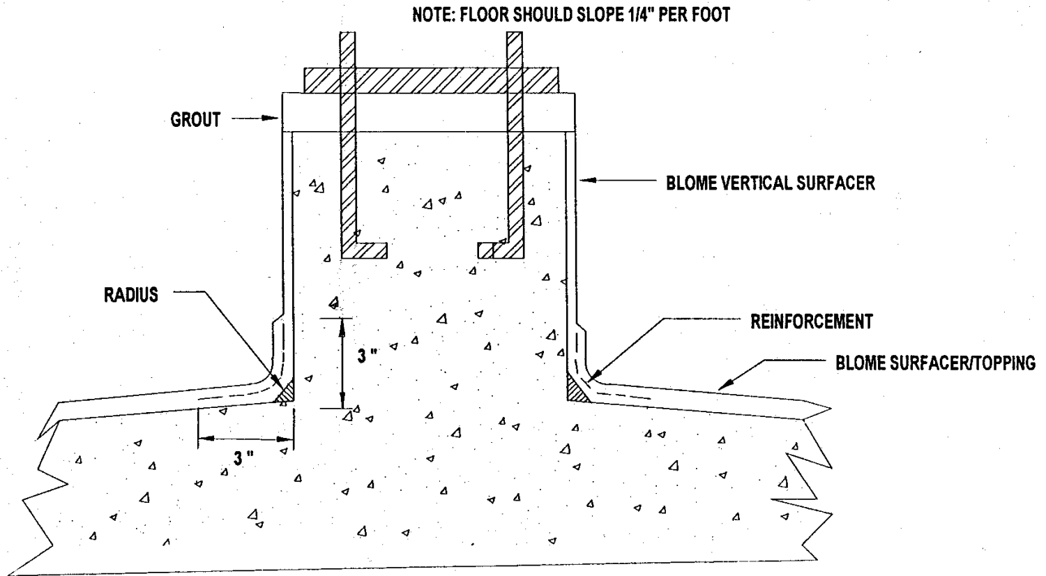
EQUIPMENT BASE WITH MONOLITHIC TOPPING AND GROUT CAP
