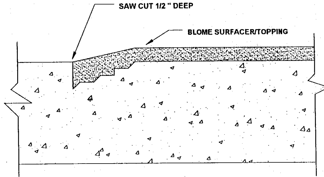
TERMINATION OF TOPPING ON CONCRETE FLOORS
