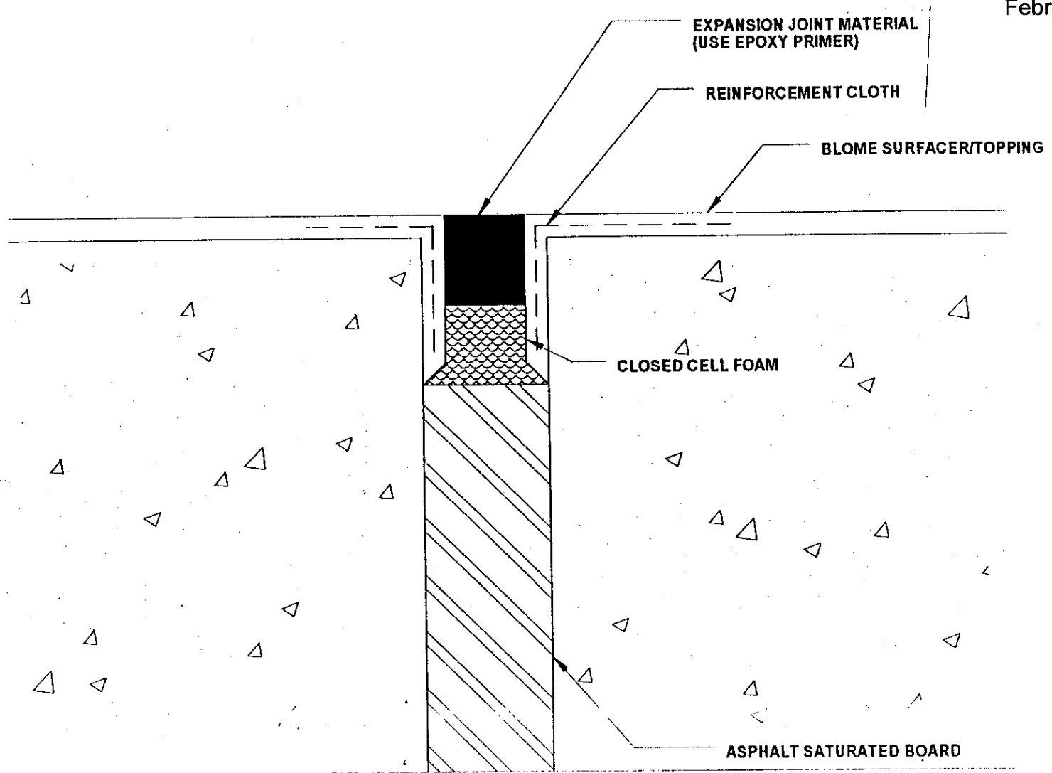
PREFERRED EXPANSION JOINT FOR MONOLITHIC TOPPINGS
