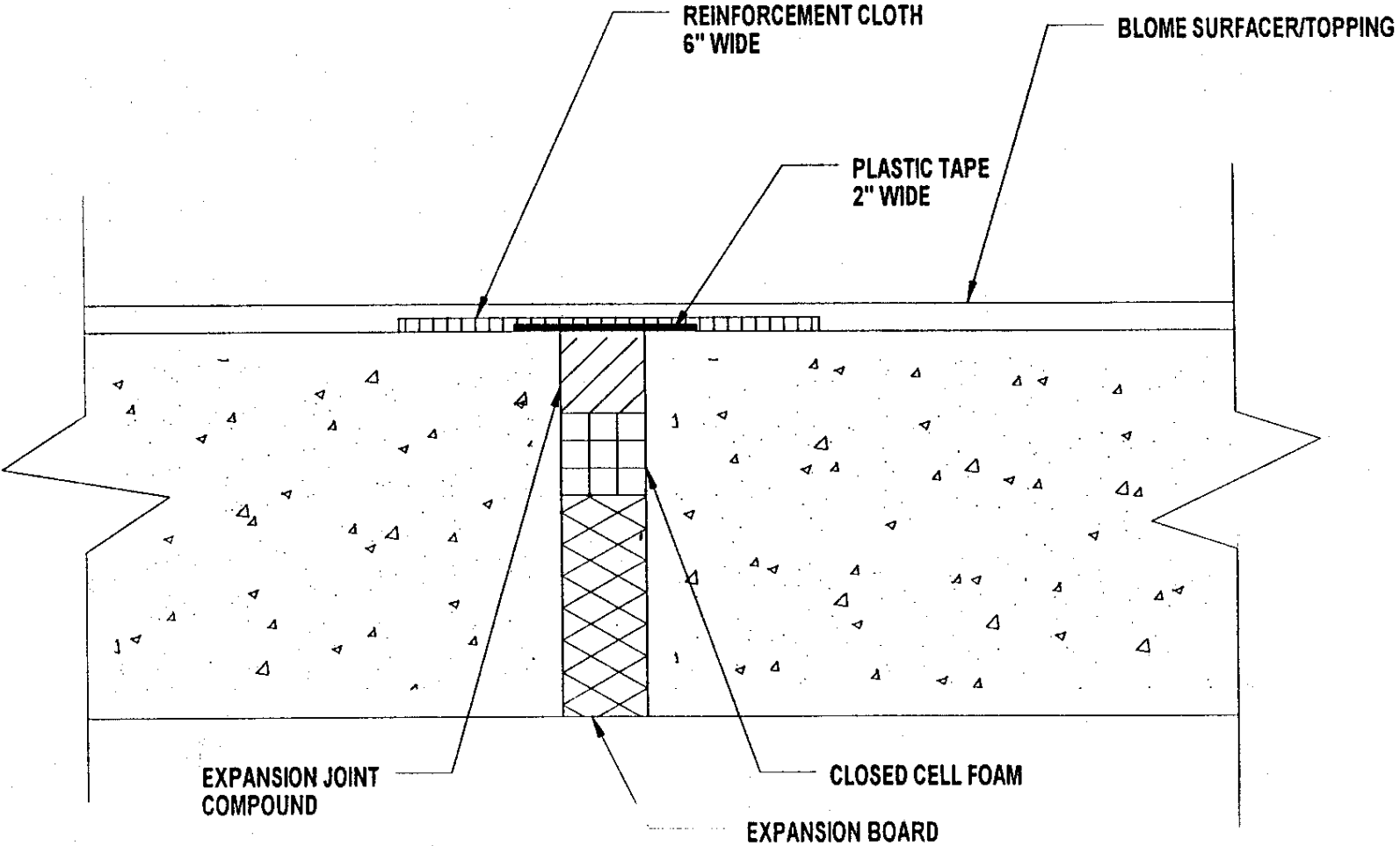
REINFORCED SURFACER OVER EXPANSION JOINTS WITH MINIMAL MOVEMENT
