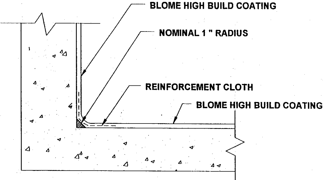
HIGH BUILD COATING FLOOR TO WALL DETAIL
