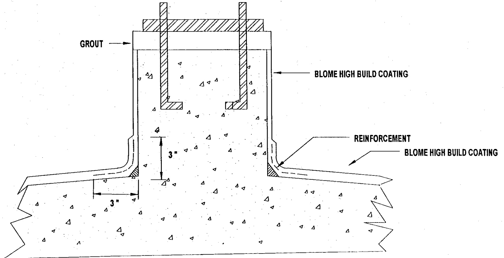
EQUIPMENT BASE WITH HIGH BUILD COATING AND GROUT CAP
